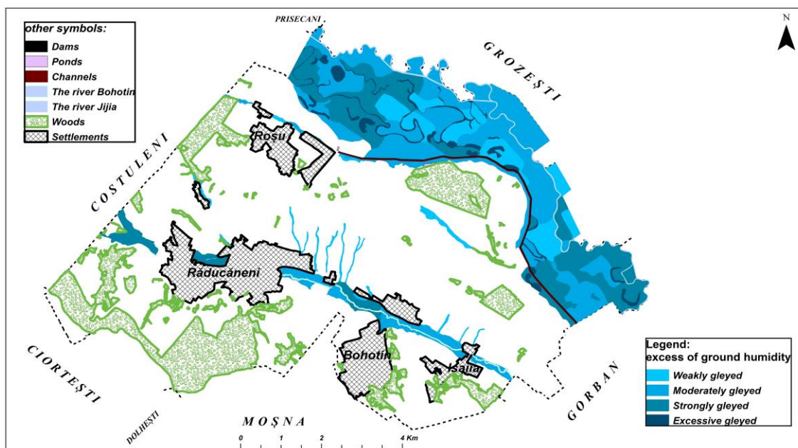
Figure 6 Gleization distribution
