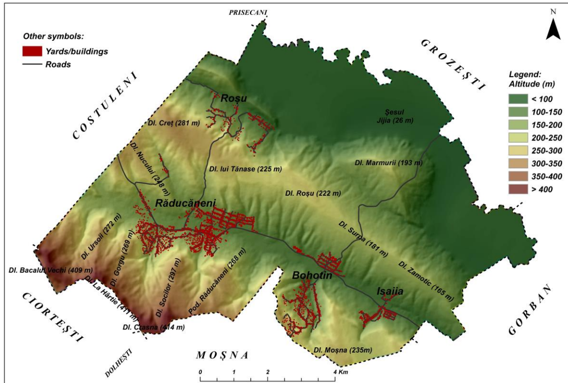
Figure 2 Altitude distribution
